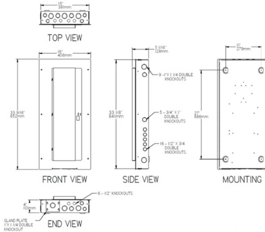
NEMA 1 Load Center Dimensions
