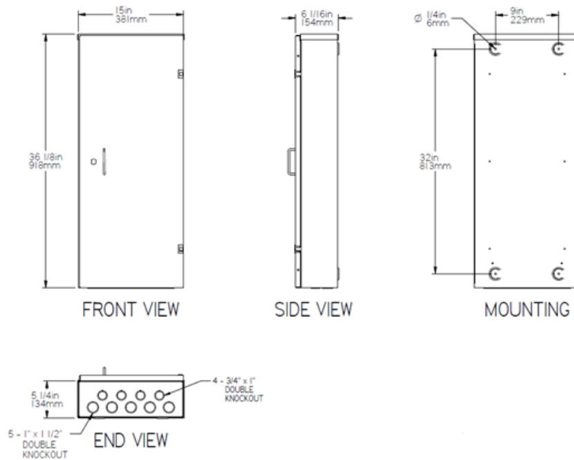
NEMA 3R Load Center Dimensions
